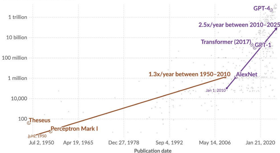
Training datapoints (datapoints)
